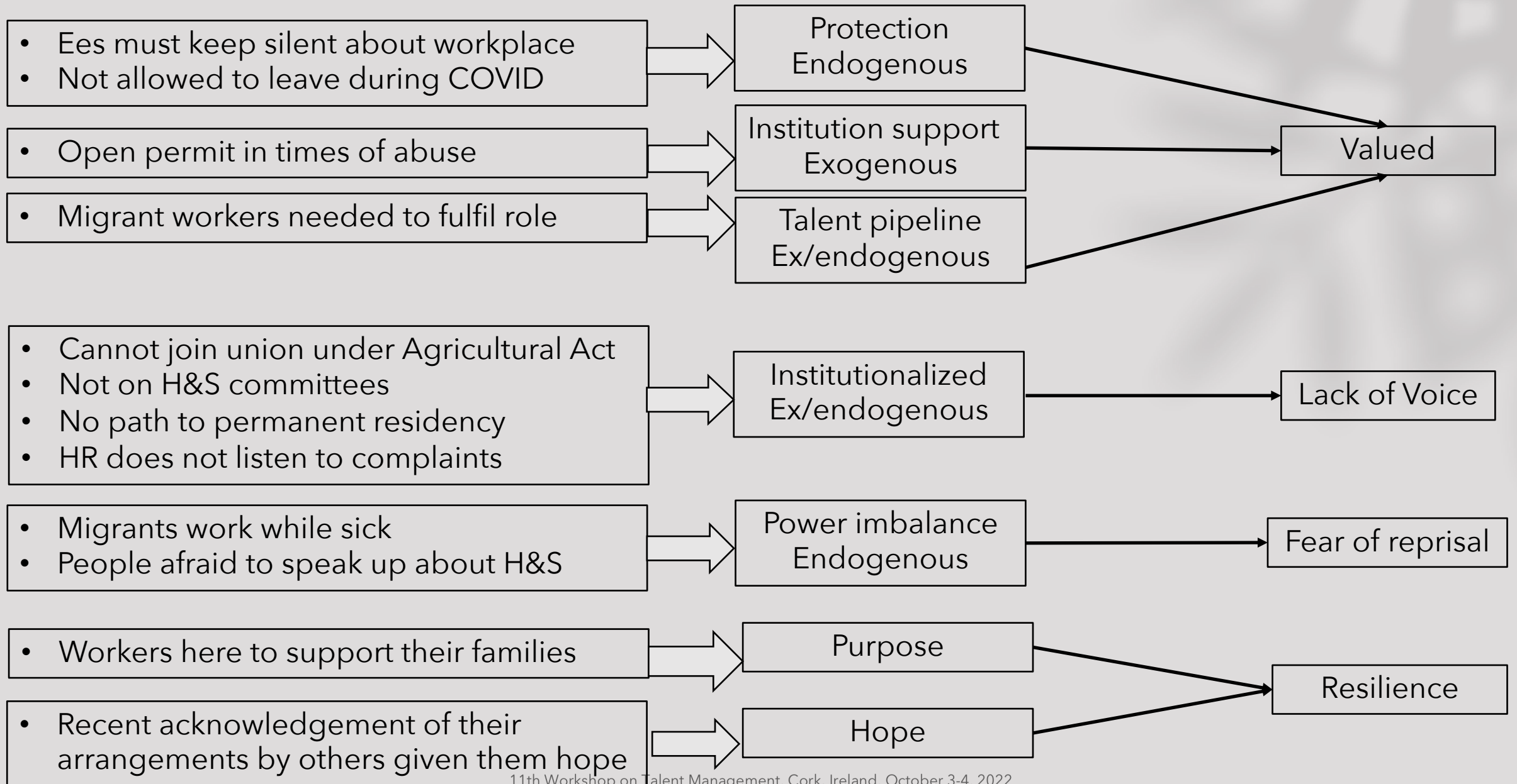
Figure 1: Data Structure
